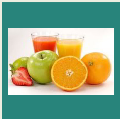
Mash Enzyme
