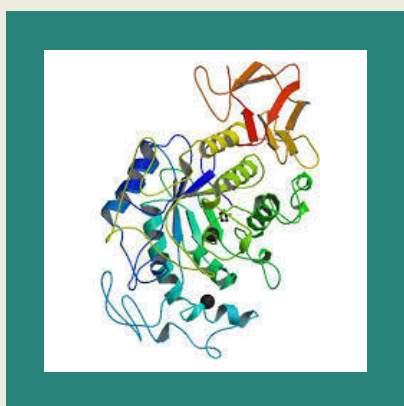
Pancreatin Enzymes
