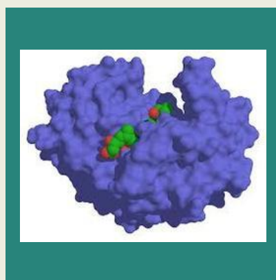
Pepsin
