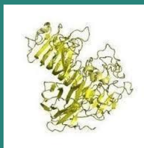
Dextranase Enzyme
