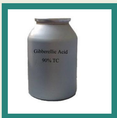
Gibberellic Acid
